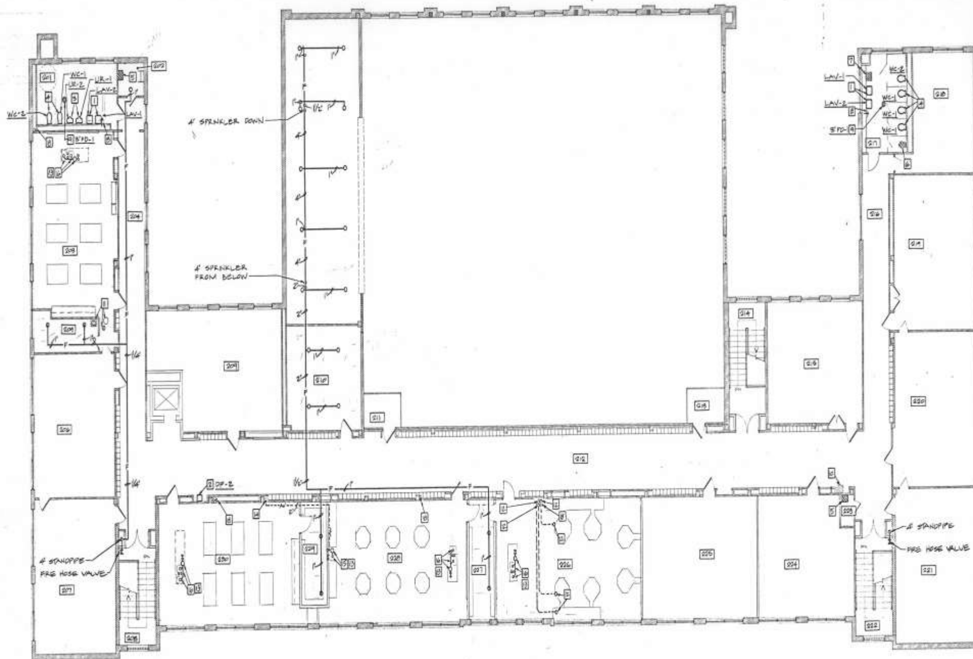
SECOND FLOOR PLAN - MAIN BUILDING
