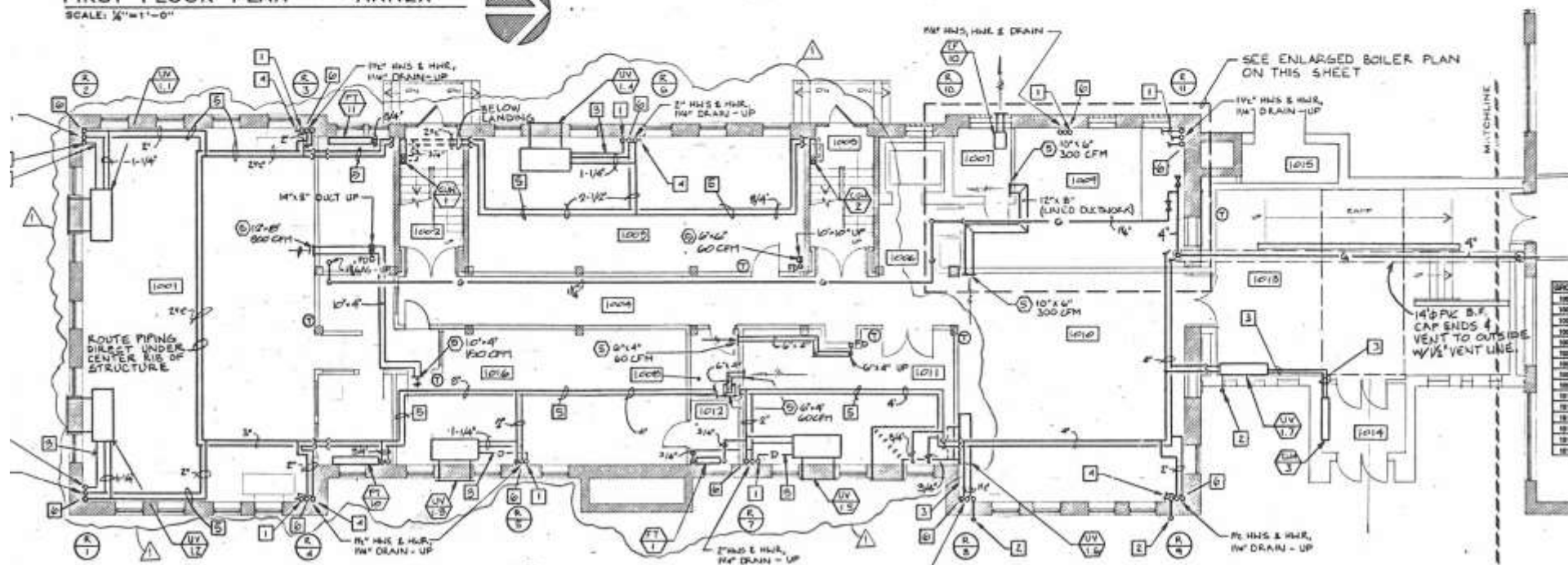
GROUND FLOOR PLAN - ANNEX
