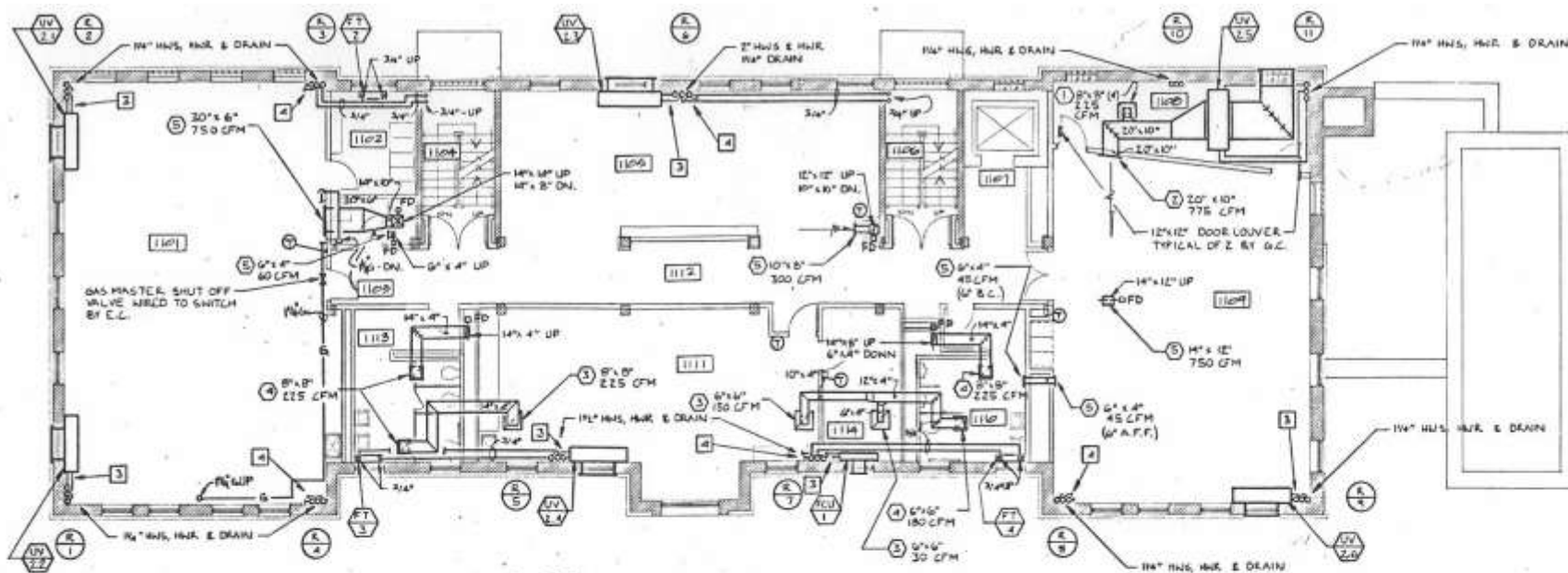
FIRST FLOOR PLAN - ANNEX
